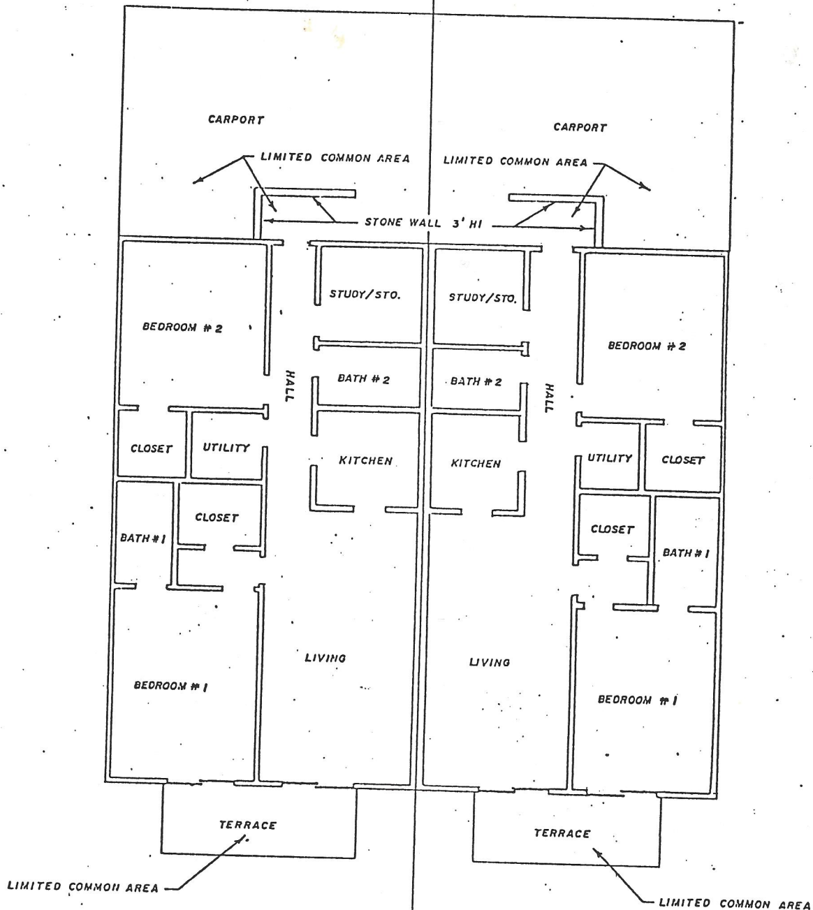
TYPICAL FLOOR PLAN Ground Level (Left Hand) 1,298 Sq. Ft.
