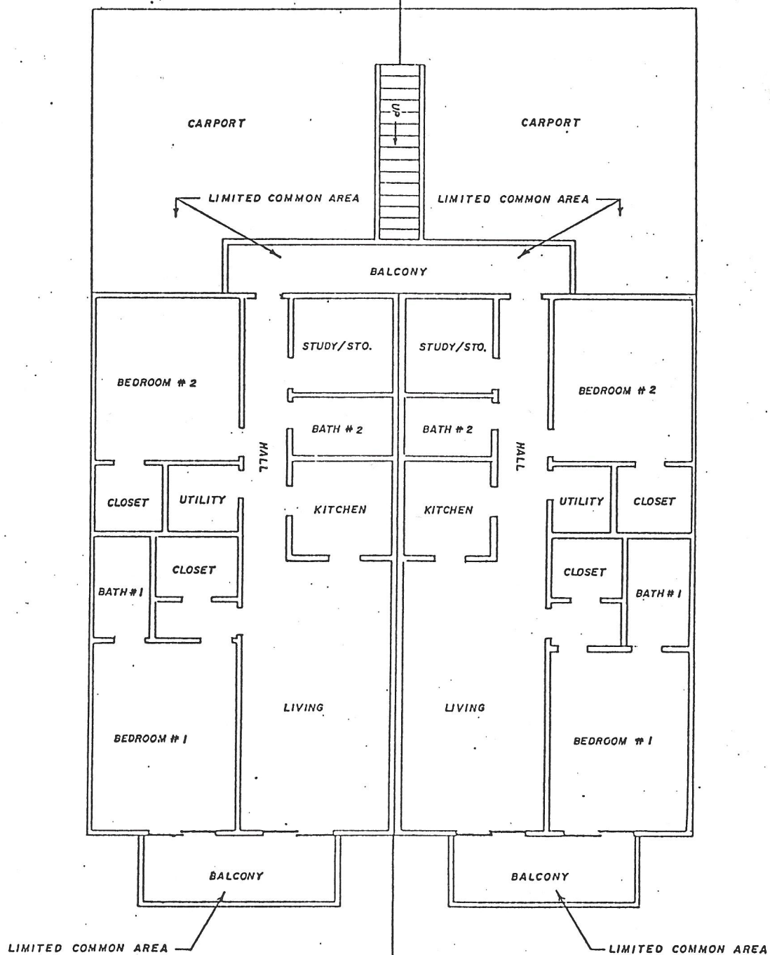
TYPICAL FLOOR PLAN Second Level (Left Hand) 1,298 Sq. Ft.
